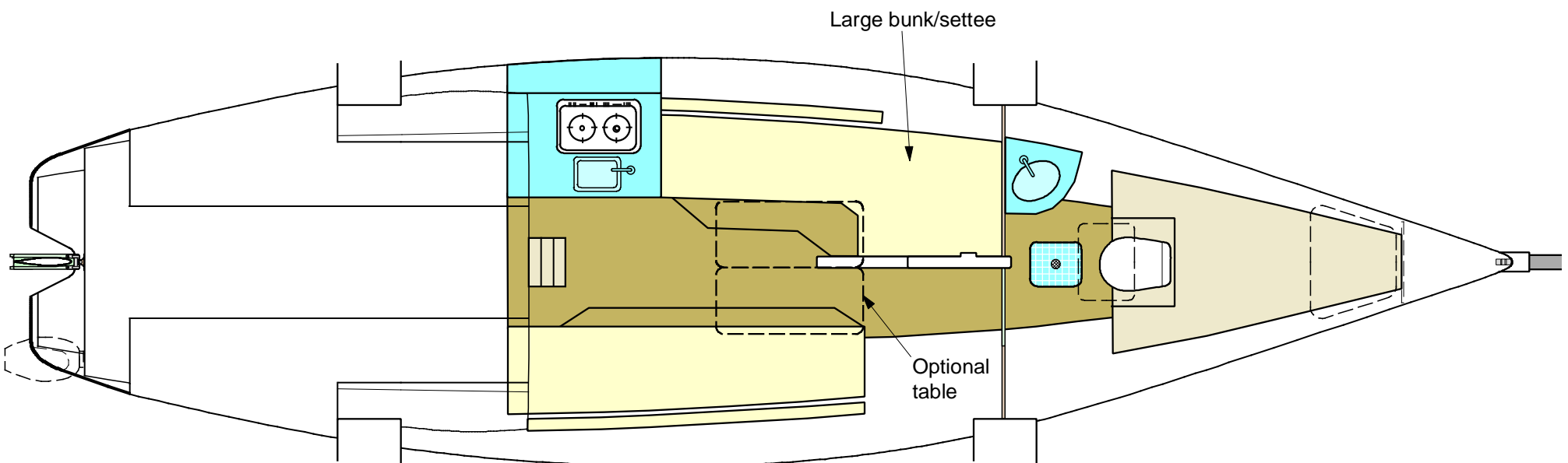
BASIC F-33ST INTERIOR With extra long cockpit
