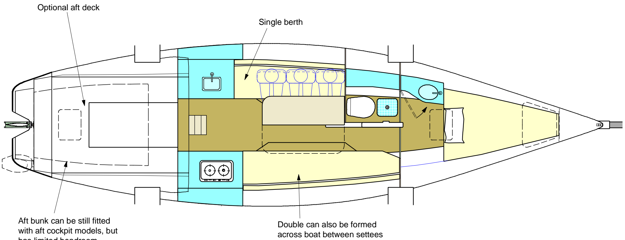
F-33 CRUISING INTERIOR Aft Cockpit Option 2
