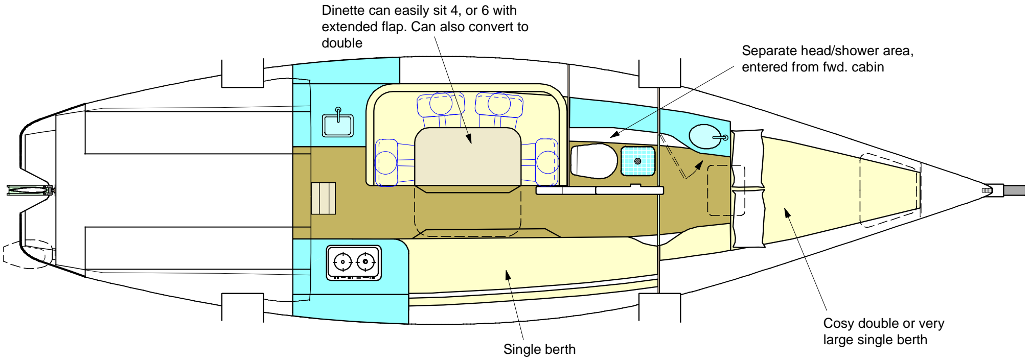
F-33 CRUISING INTERIOR Aft Cockpit Option 1
