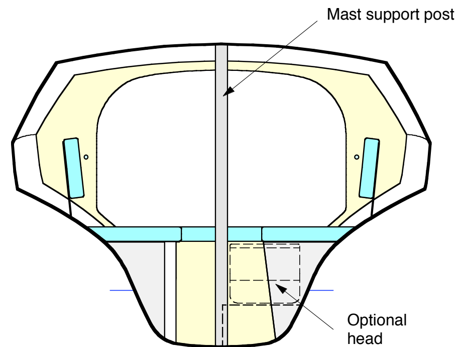
INTERIOR SECTION (Looking aft)
