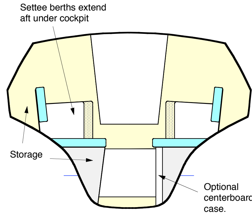
INTERIOR SECTION (Looking aft)
